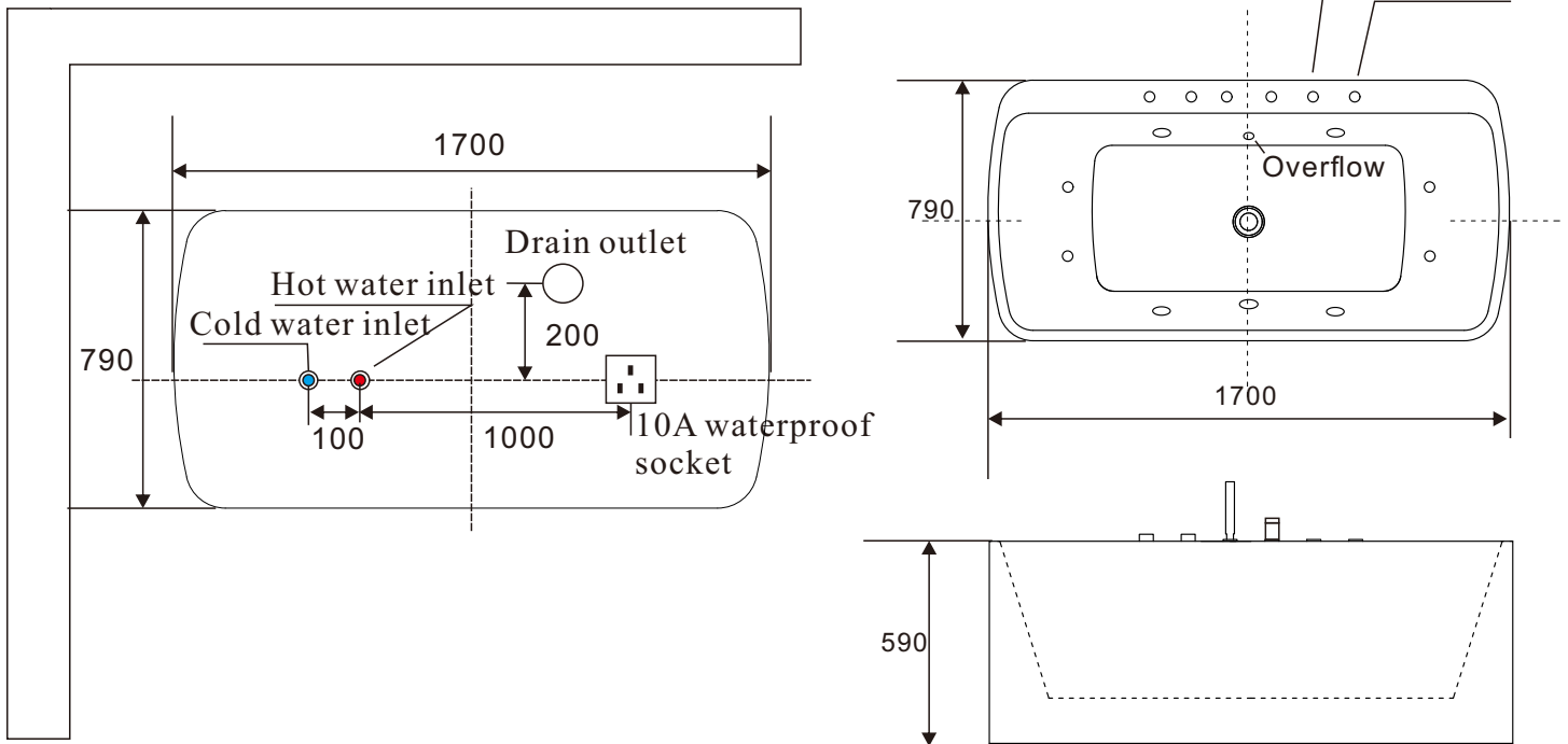
Three dimension erection size drawing
